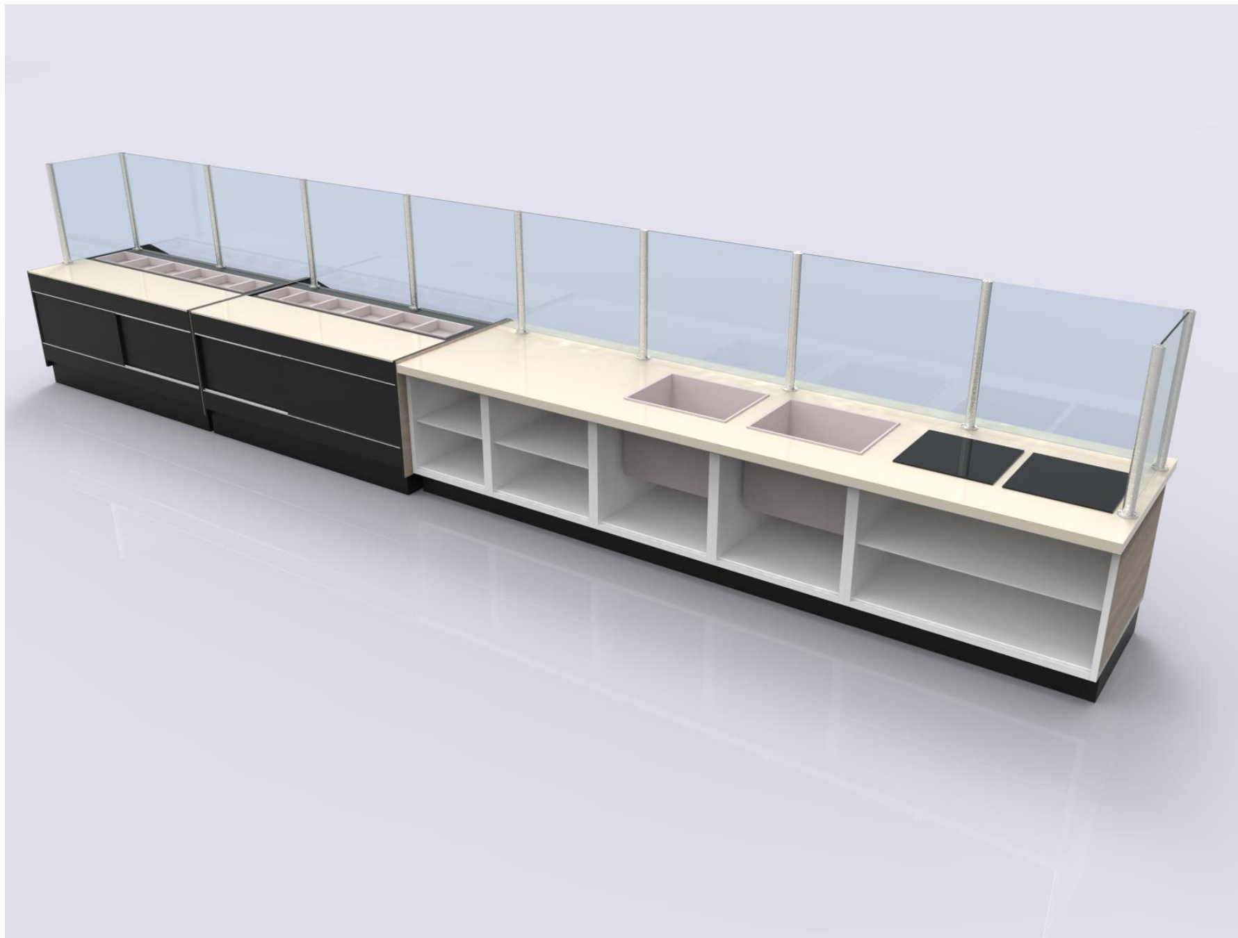
Example C - QSR Cabinet w/Bin Drop-in, Sneeze Guard, Floating Fronts and Cooler Case (by others)
