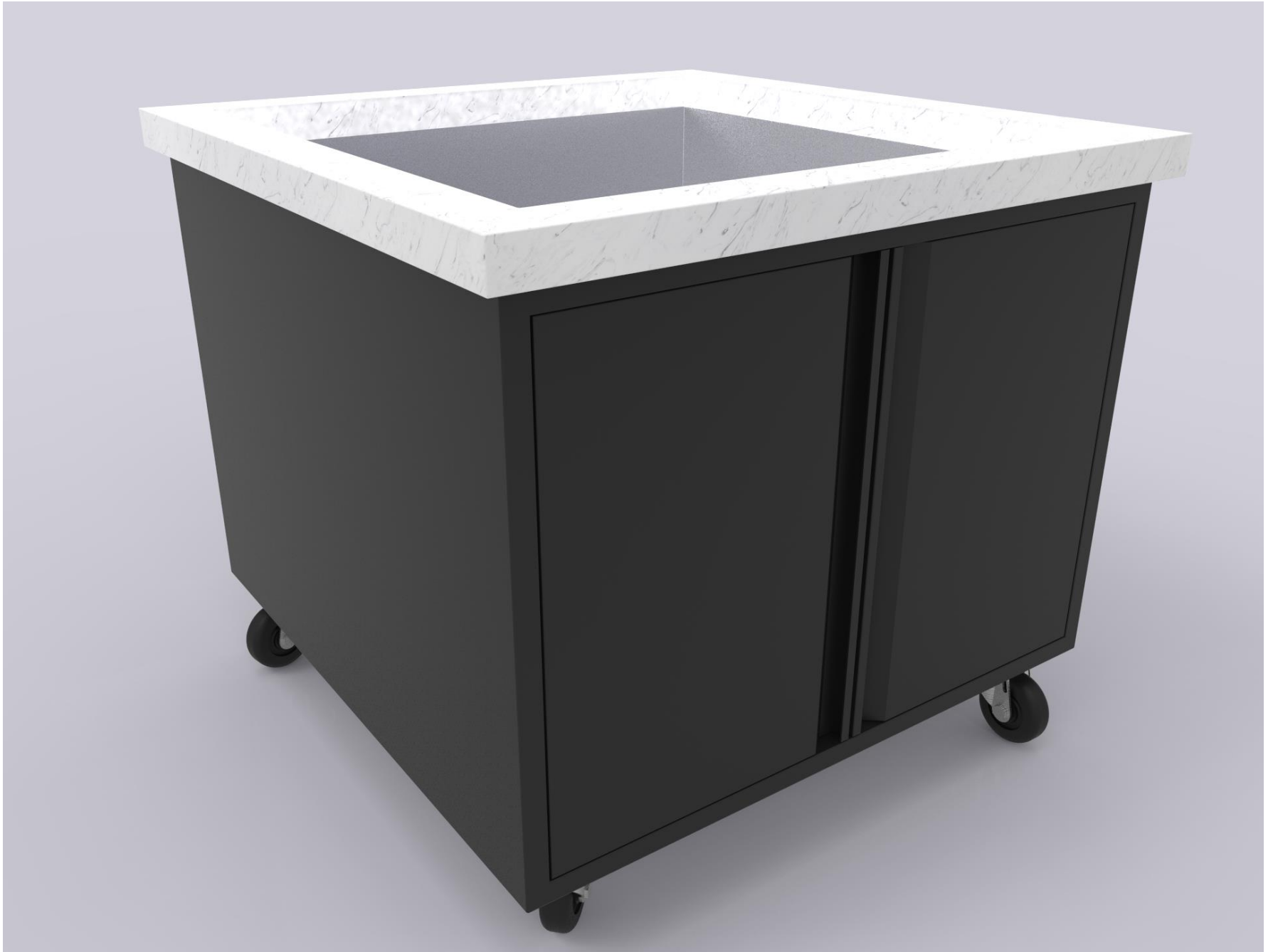
Example I - Specialty Fixtures: Iced Beverage Tub, w/Solid Surface Top Trim & 2" Drop Edge
